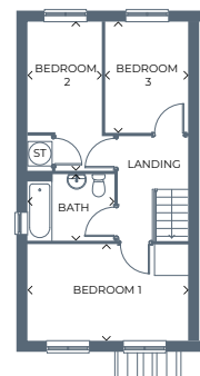
First floor
